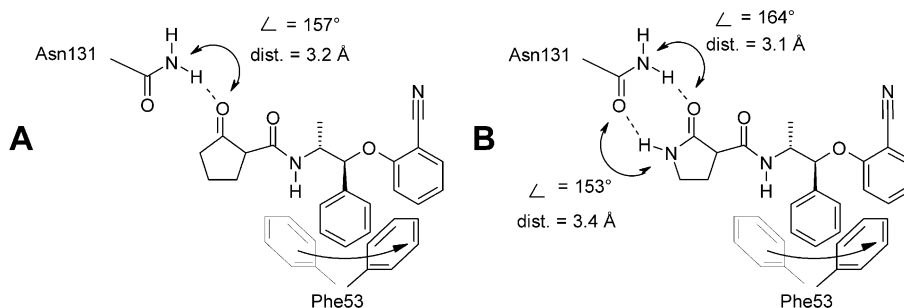
Figure 2. Schematic representation of cyclopentanone (A) and butyrolactam (B) binding interactions with Asn131. Phe53 is displaced away from the cyclopentanone and butyrolactam rings by the inhibitor phenyl substituent.
