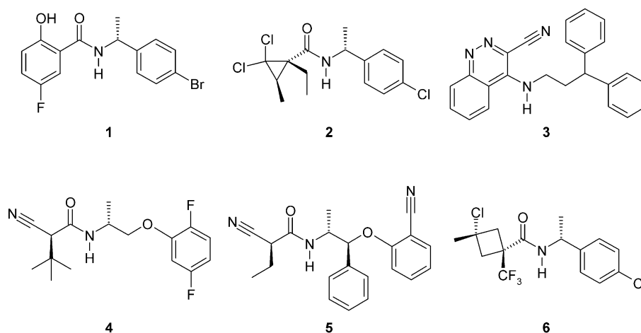
Figure 1. Inhibitors that have been co-crystallized with SD for structure determination by X-ray diffraction.
